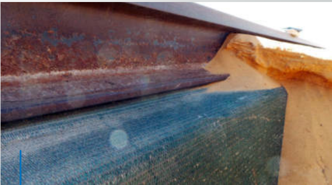
Resilient pad between rail and beam – no ingress of sand
